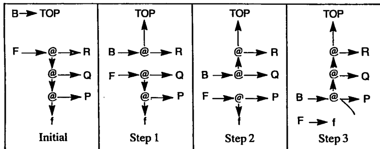
Figure 11.3 Pointer-reversal in action on (f P Q R)
