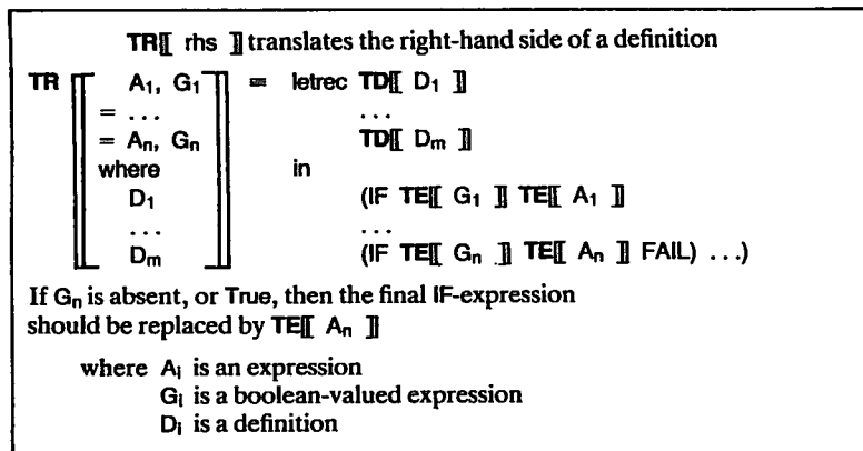
Figure 4.2 The final TR translation scheme
