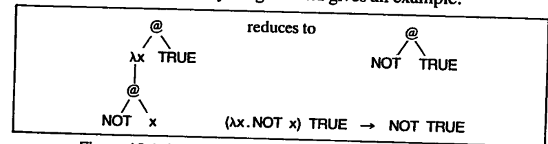
Figure 12.1 Instantiating the body of a lambda abstraction
