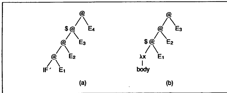
Figure 11.1 Finding the next redex (marked $)
