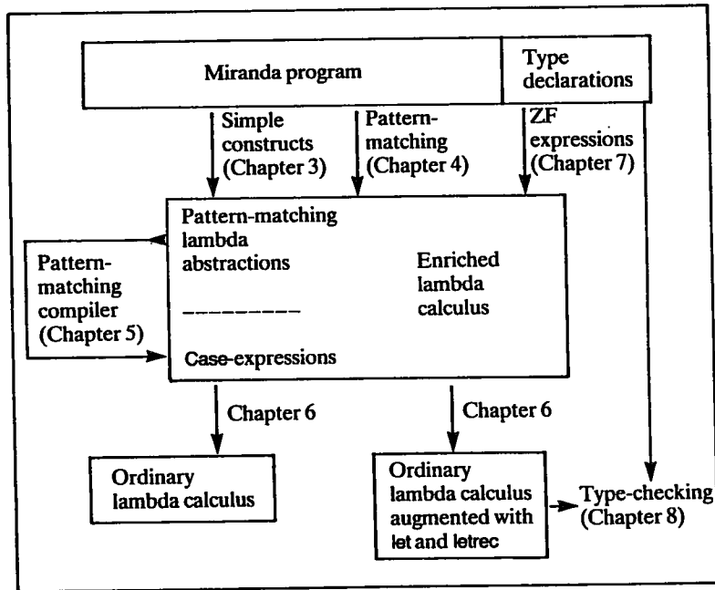
Figure 3.4 Organization of Chapters 4–8
