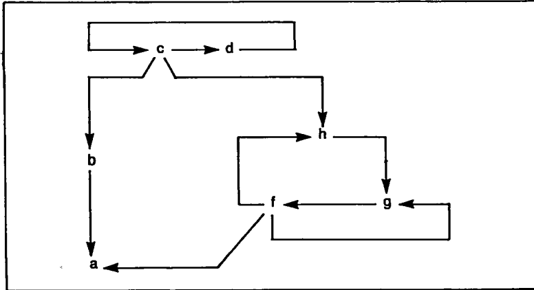
Figure 6.4 Example dependency graph
