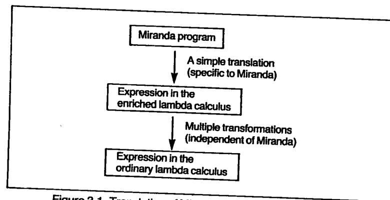
Figure 3.1 Translation of Miranda into the lambda calculus
