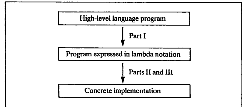
Figure 1.1 Implementing a functional program
