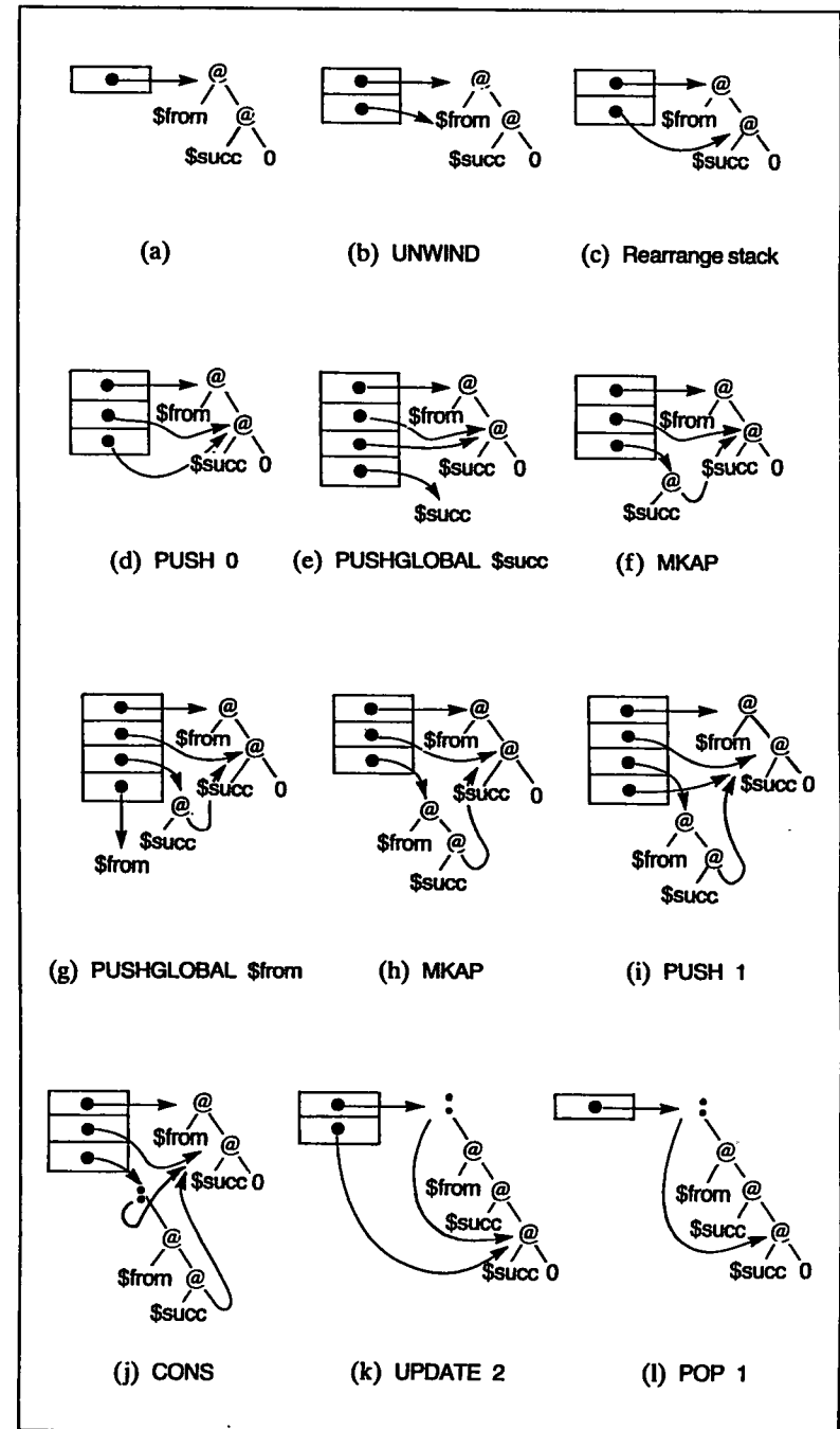
Figure 18.2 Evaluation of (\$from (\$succ 0))
