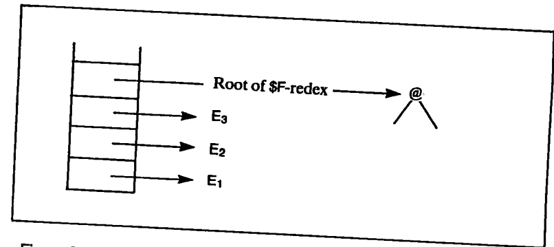
Figure 21.2 Current context on entry to three-argument supercombinator W
