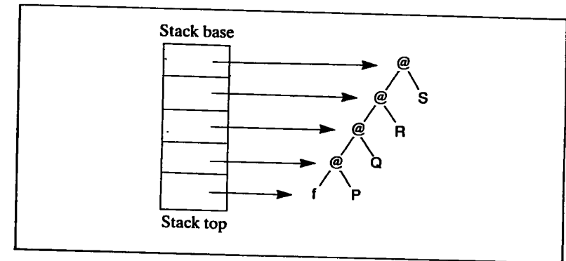
Figure 11.2 The spine stack
