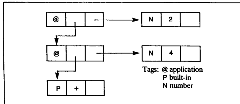
Figure 10.4 The concrete tree of (+ 4 2)
