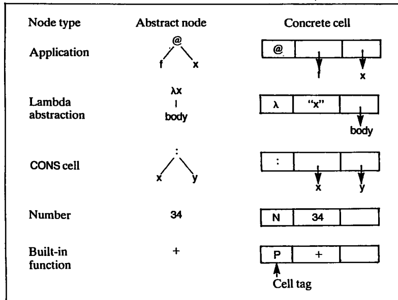
Figure 10.3 Possible concrete representations
