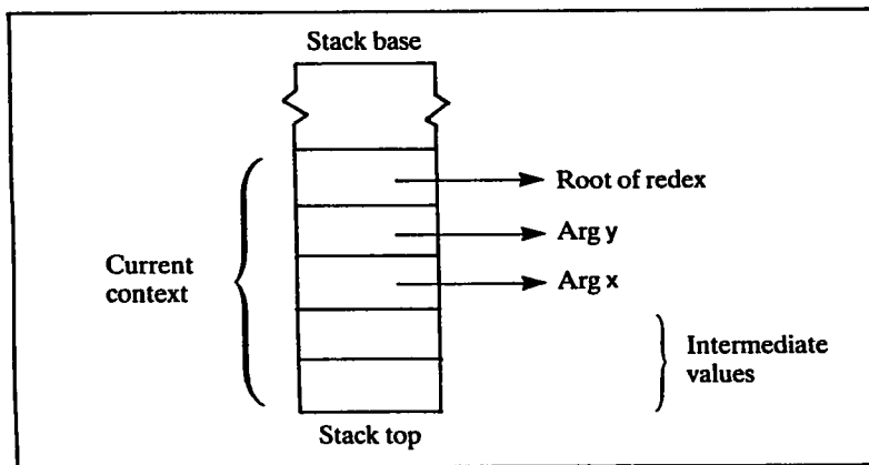
Figure 18.6 An example context
