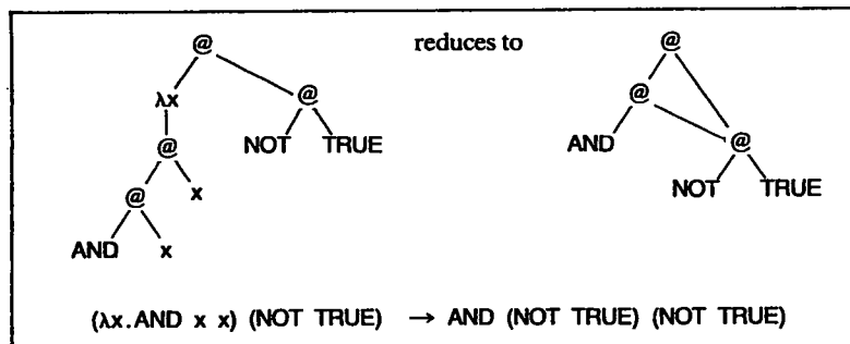
Figure 12.2 Pointer substitution
