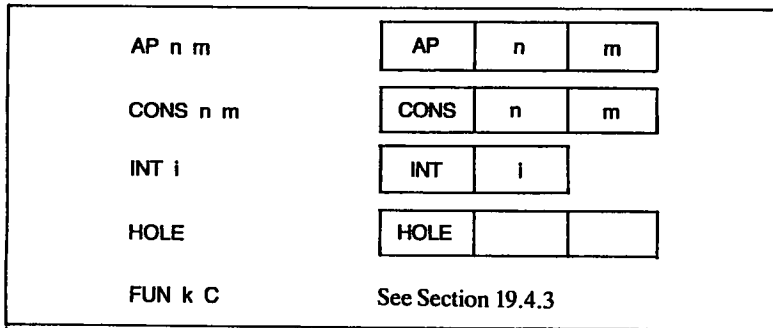
Figure 19.3 Node representations in the G-machine
