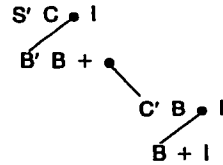
Combinator representation
