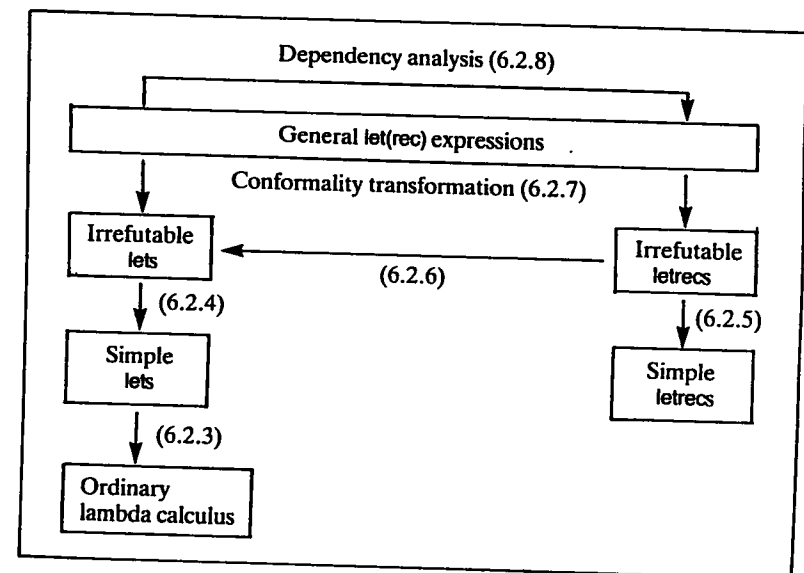
Figure 6.3 Map of \text{let}(\text{rec}) transformations
