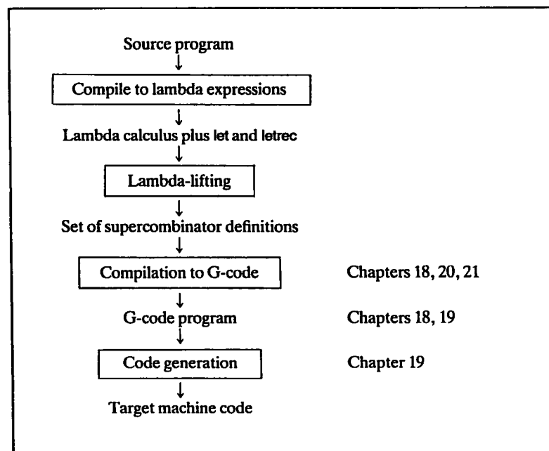
Figure 18.1 Structure of the G-machine compiler
