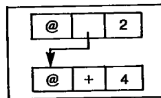
Figure 10.5 The concrete tree of (+ 4 2) (unboxed representations)
