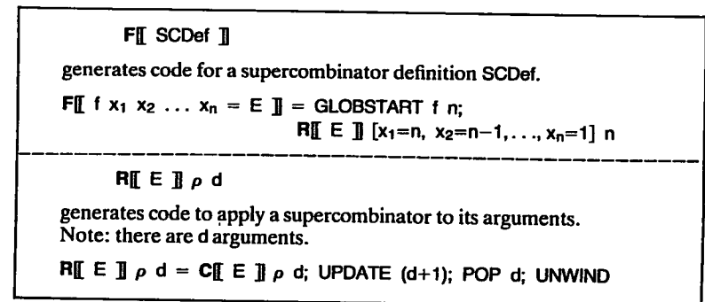
Figure 18.7 The R compilation scheme
