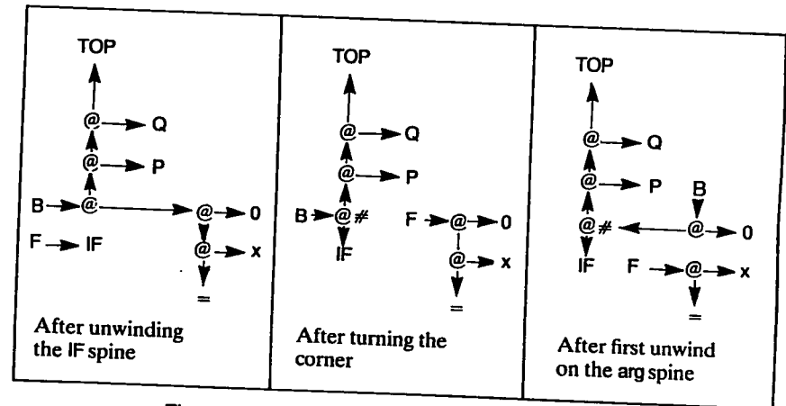
Figure 11.4 Pointer-reversal for argument evaluation
