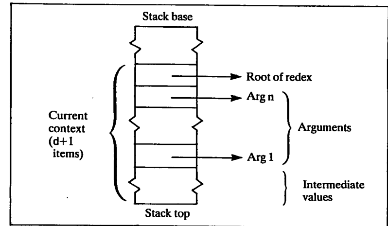
Figure 18.5 The stack during G-code execution
