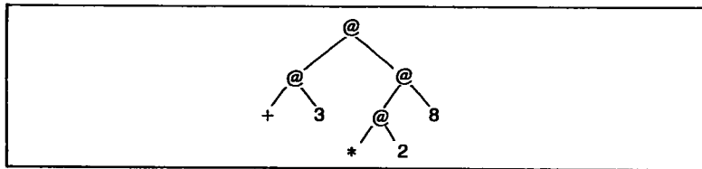
Figure 10.1 The tree of (+ 3 (* 2 8))
